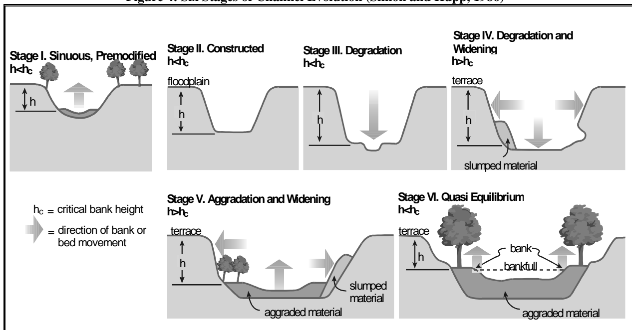
Figure 4: Six Stages of Channel Evolution (Simon and Hupp, 1986)
